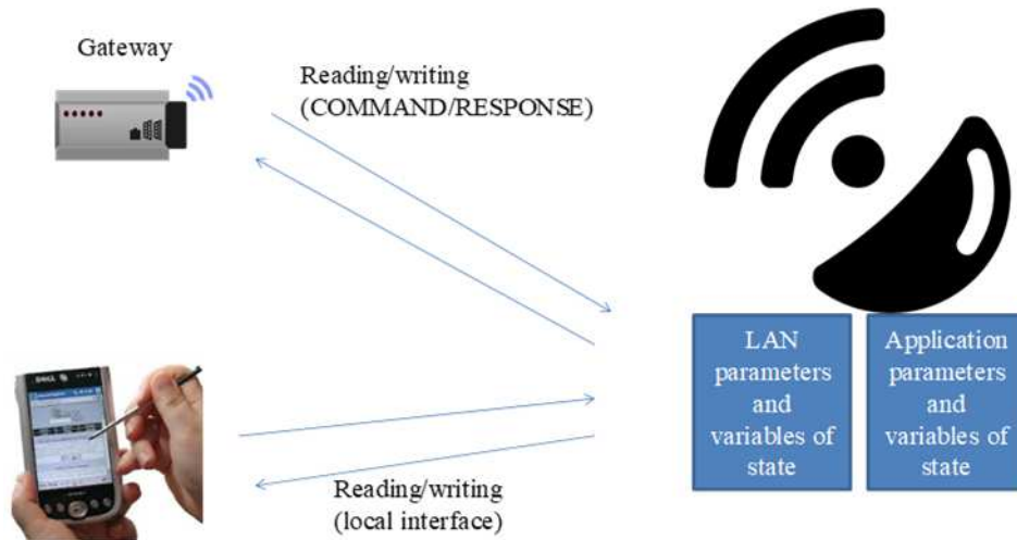
Figure 1 : Configuration model
